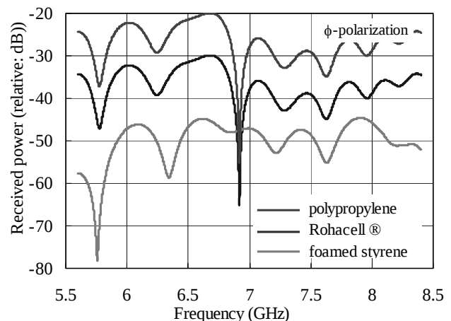
Fig. 4 Reflection characteristics of turn tables of different materials
