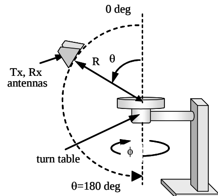
Fig. 3 Measurement of the reflected wave from a turn table
